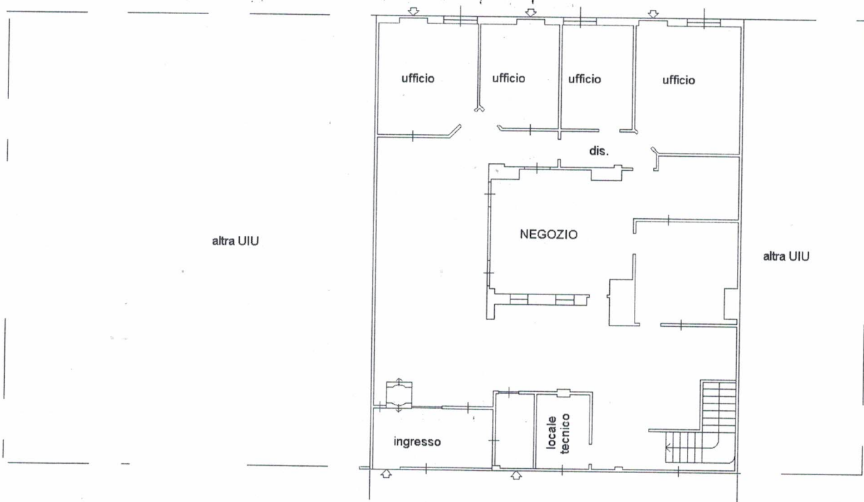
PIANO TERRA H 3,50
