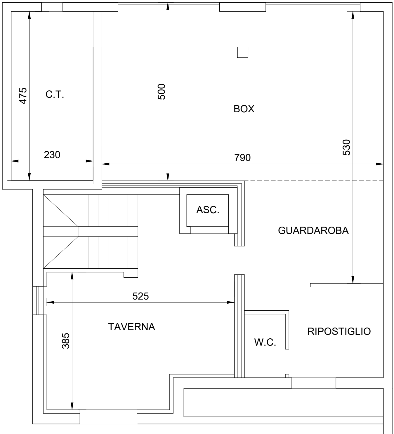
PIANO INTERRATO
